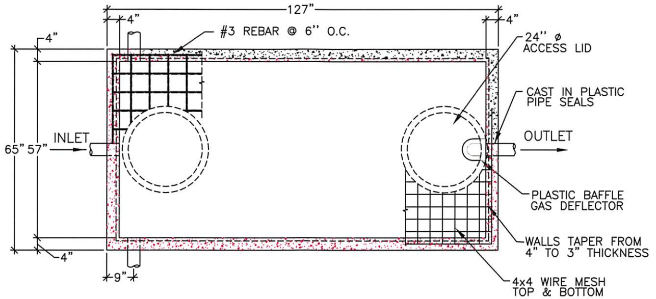
PLAN VIEW
