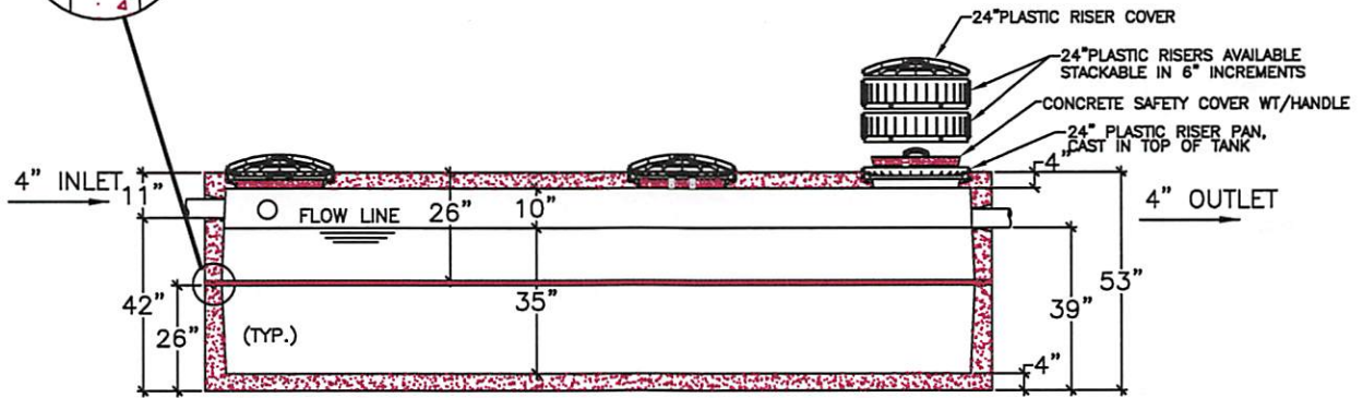
SECTION VIEW
