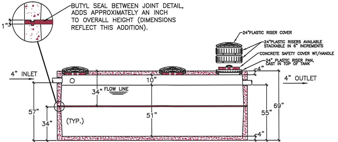
SECTION VIEW
