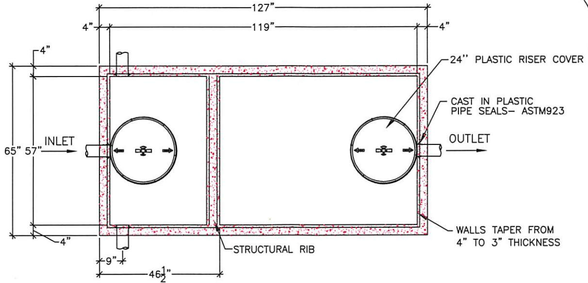
PLAN VIEW
