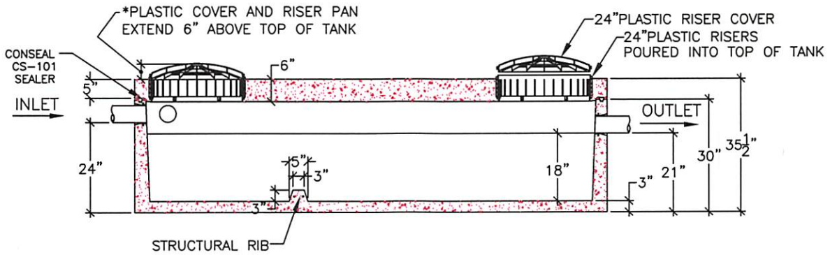
SECTION VIEW
