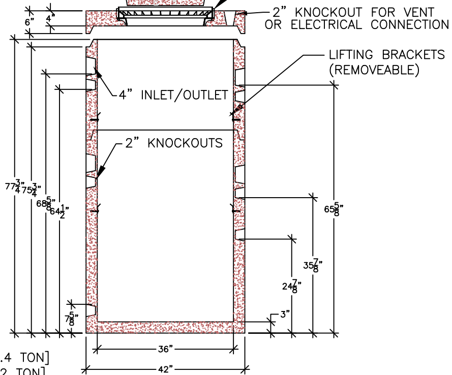
SECTION VIEW
