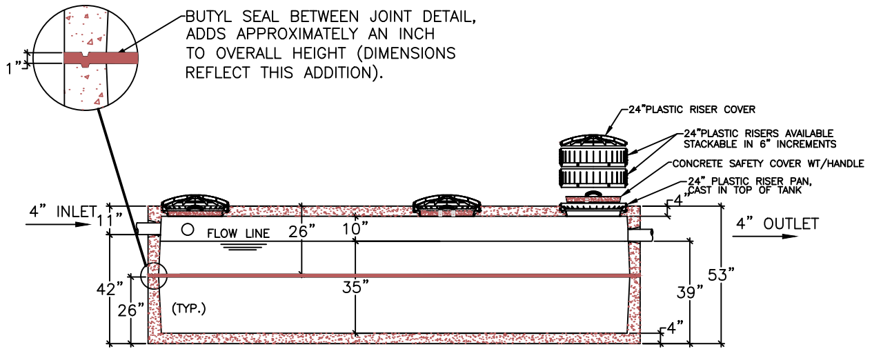
SECTION VIEW
