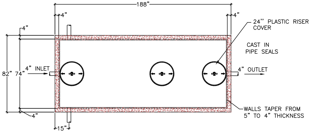
PLAN VIEW
