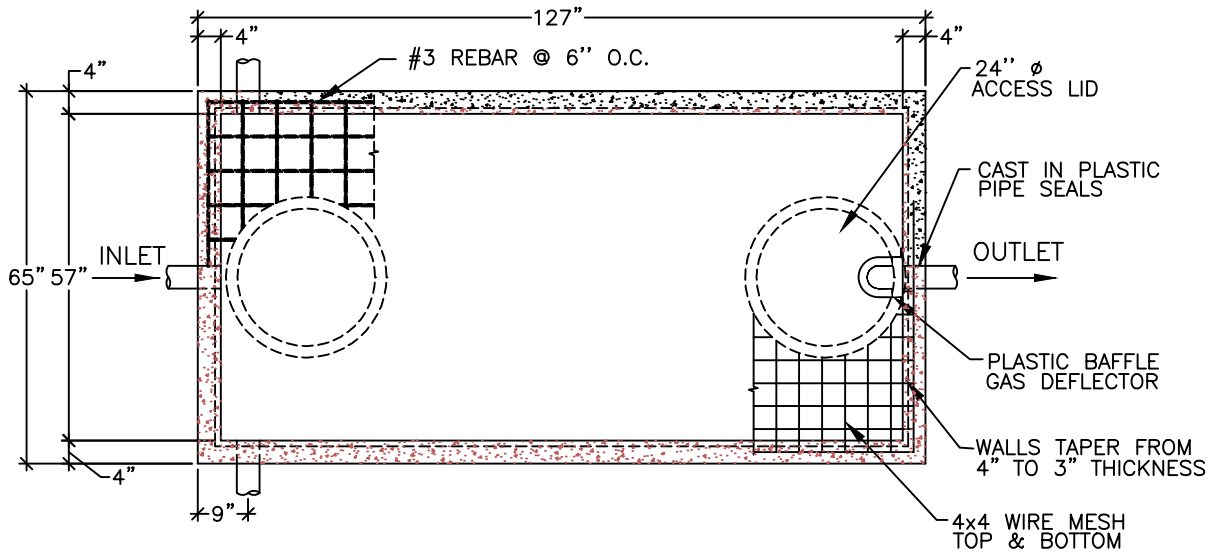
PLAN VIEW
