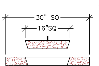
OPTIONAL COVER NOT FOR H-20 APPLICATIONS
