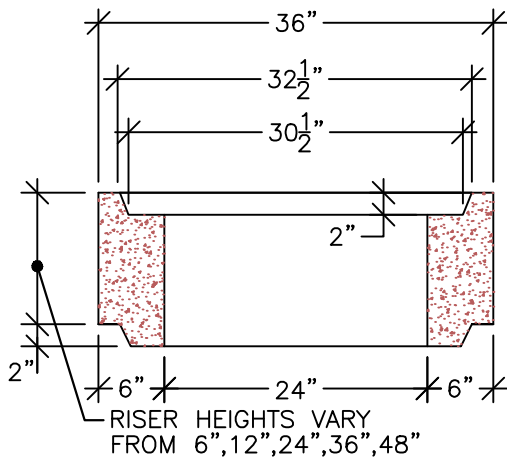
RISER (OPTIONAL)
